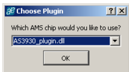
Figure 7: Plugin selection
